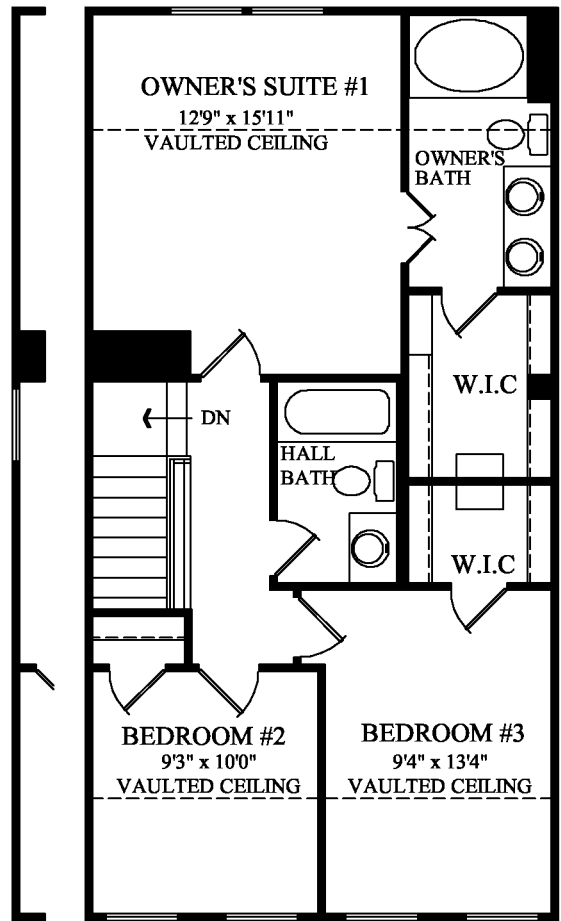
Optional Second Level
