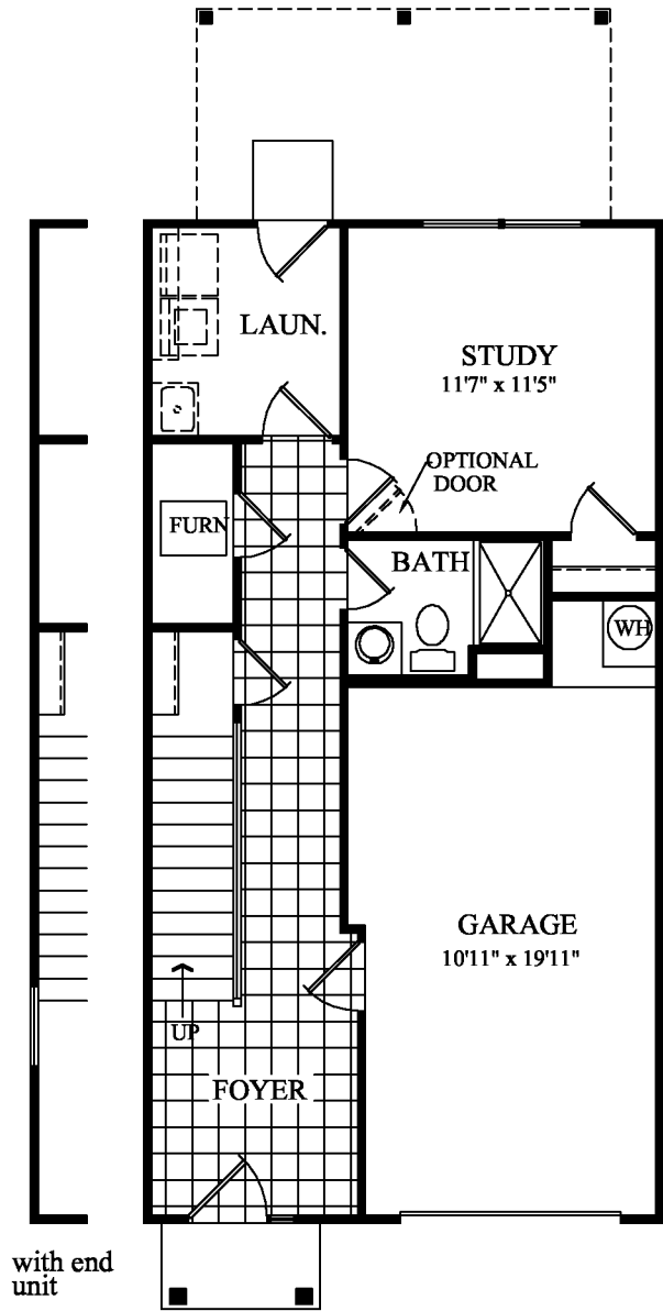
Lower Level w/ front entry garage
