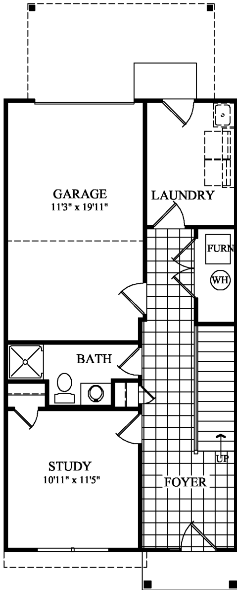
Lower Level w/ rear entry garage
